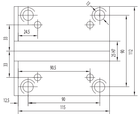
128-42508-IC 25x25 mm I.Coolant
