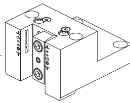
128-42508-IC 25x25 mm I.Coolant
