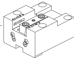
128-32506-IC 25x25 mm I.Coolant
