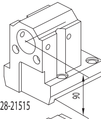
Toolholder for boring bar
