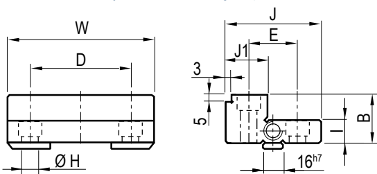
Art. 8050 Ganasia fissa con gradino piccolo e grande Fixed jaw with small and large step
