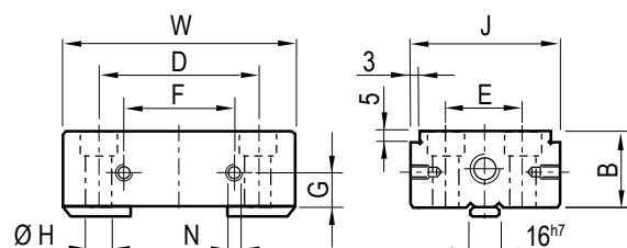
Art. 805F (Montata su Art. 866) (Assembled on Art. 866)
